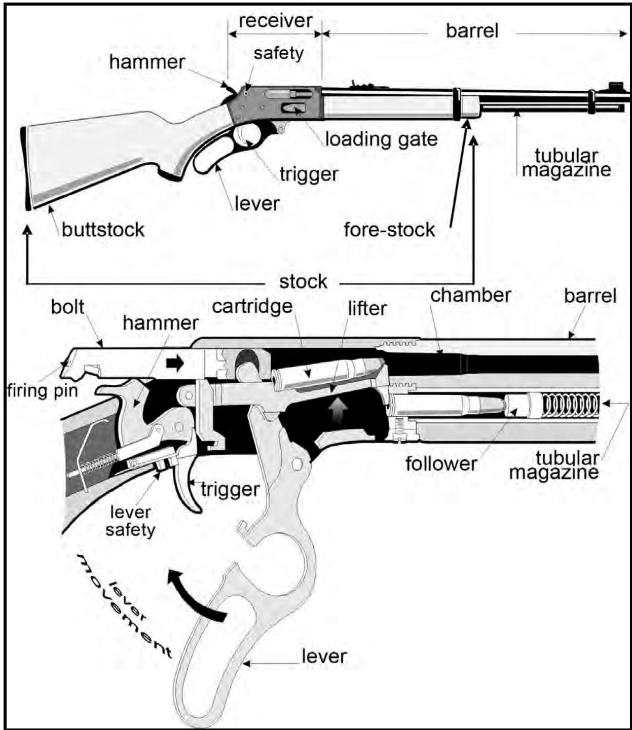
Figure 53. Lever action
