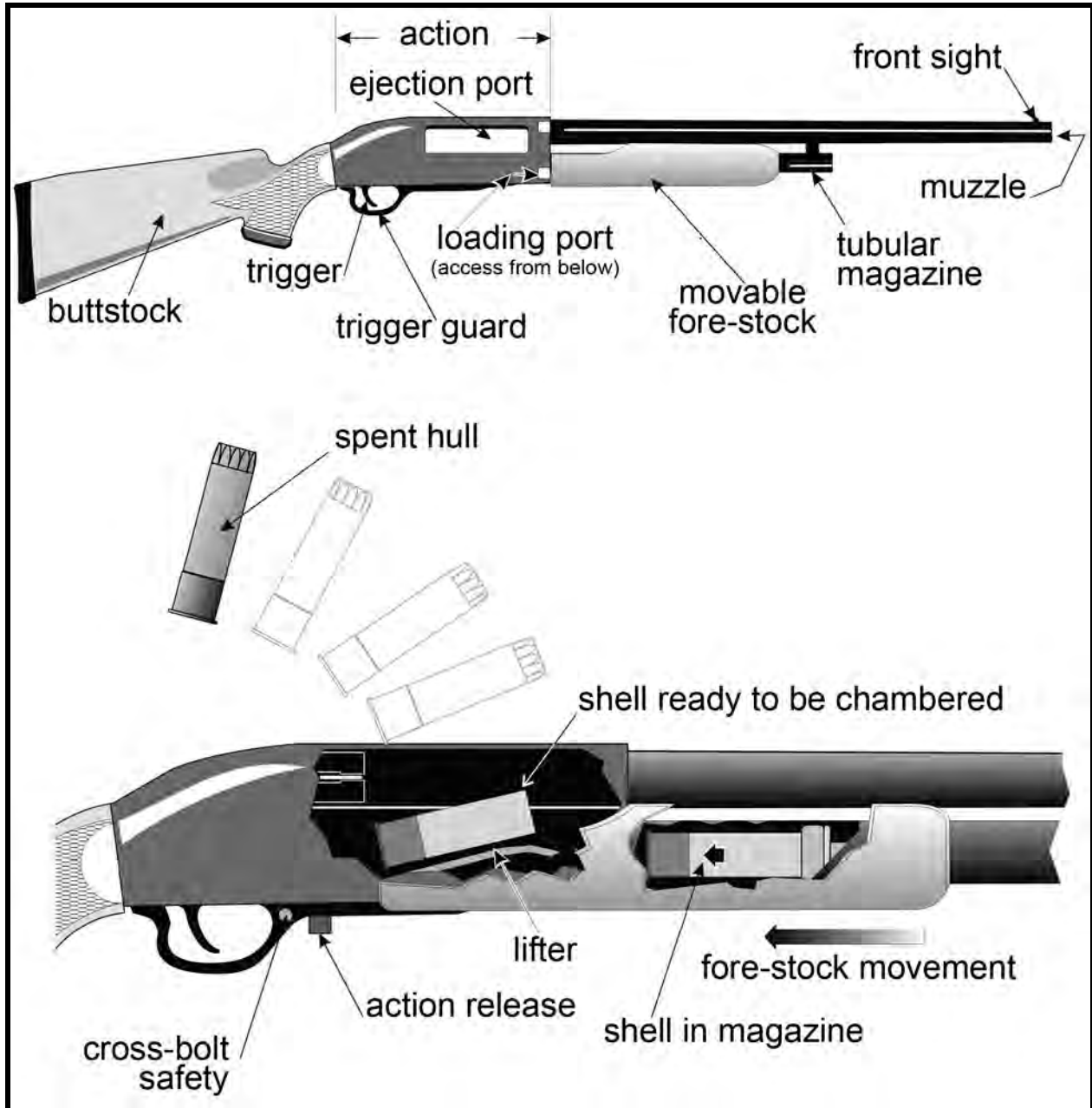
Figure 54. Pump action
